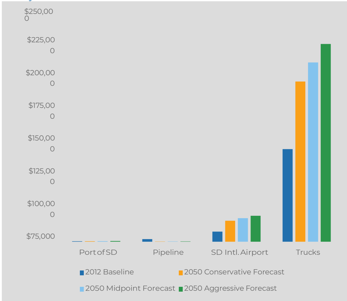
Figure 3.13: Summary of Domestic Freight Flows within, from and to San Diego County in Value: 2050 Forecast
