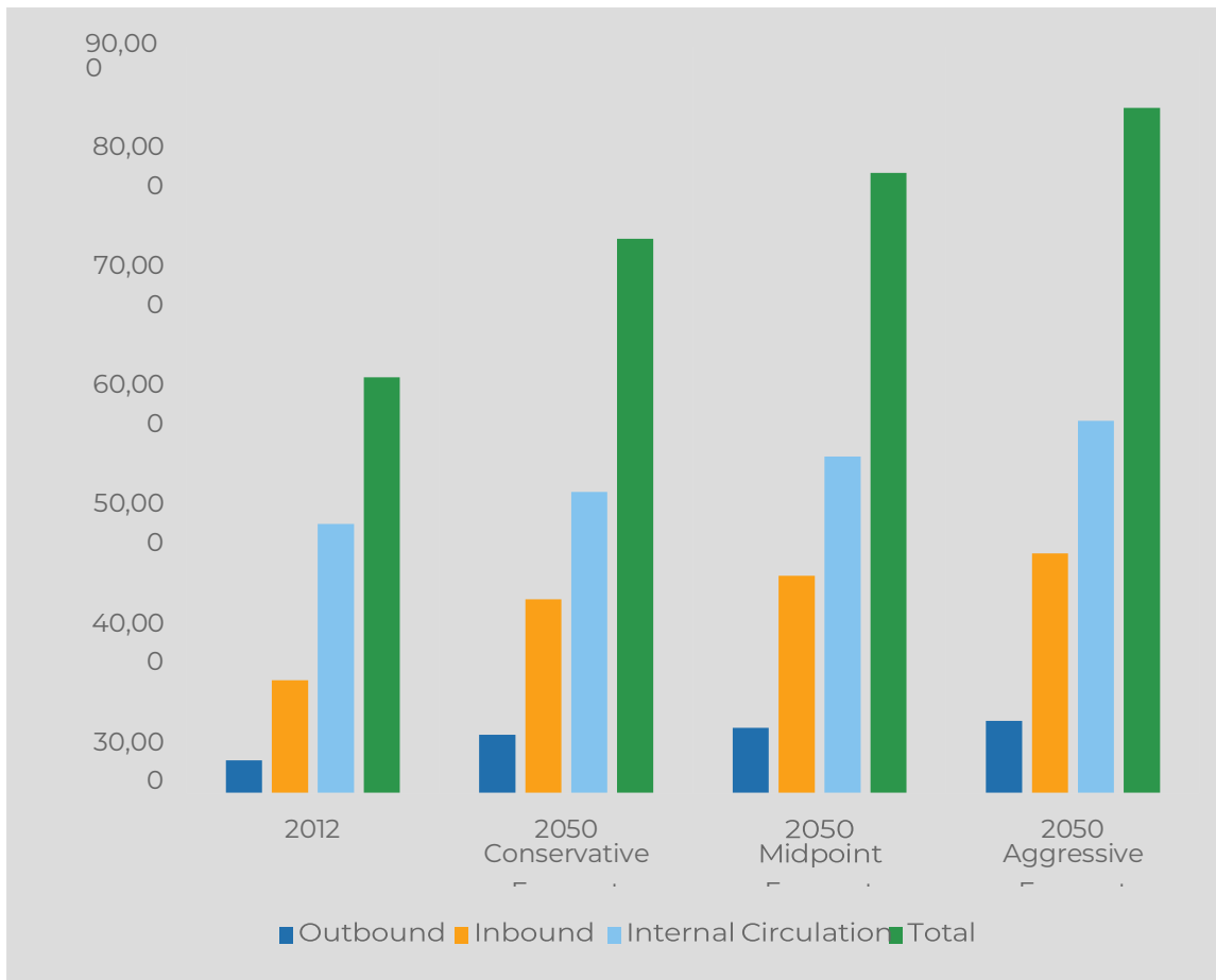
Figure 3.14: Summary of Domestic Truck Freight Flows within, from and to San Diego County and Comparison to the Region’s International Gateways: 2050 Forecast
