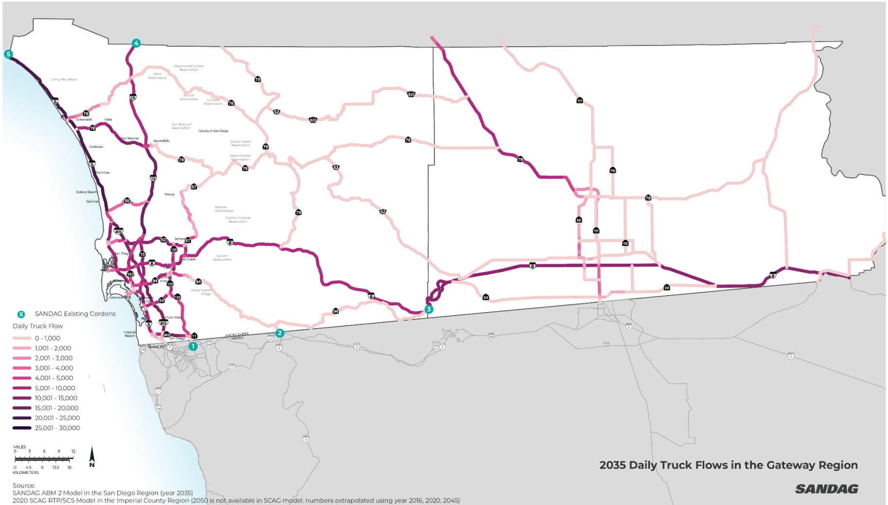
Figure 3.2: 2035 Daily Truck Volume (Preliminary Draft)
