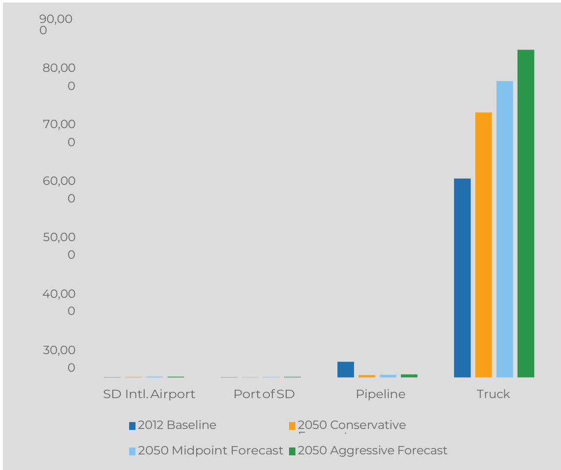
Figure 3.12: Summary of Domestic Freight Flows within, from and to San Diego County in Volume: 2050 Forecast
