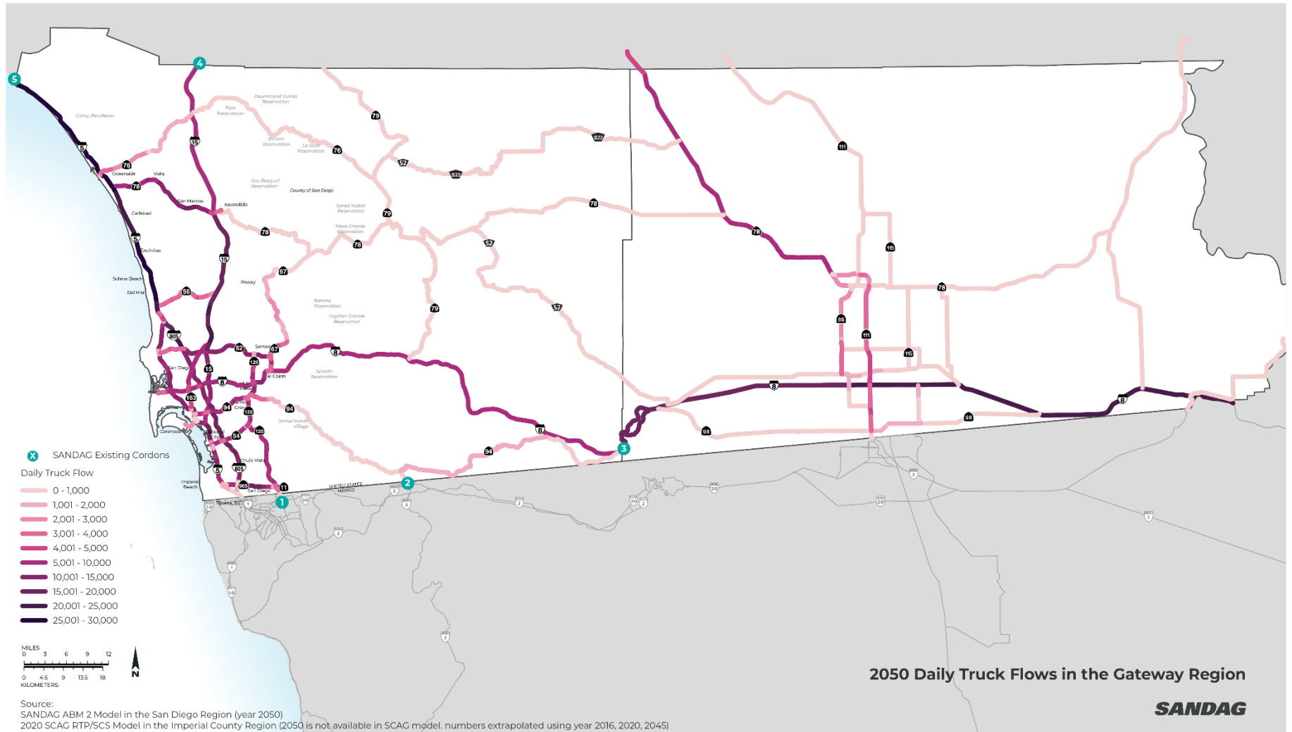
Figure 3.3: 2050 Daily Truck Volume (Preliminary Draft)
